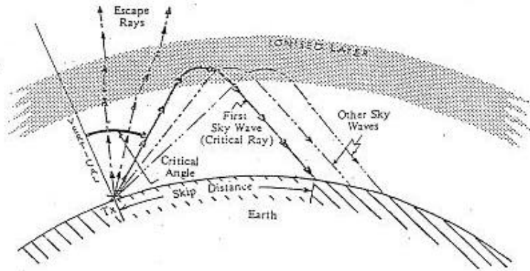
Figure 4 – Critical angle (HF band)
