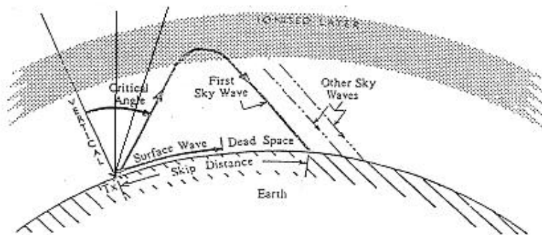
Figure 5 – Dead space (HF band)
